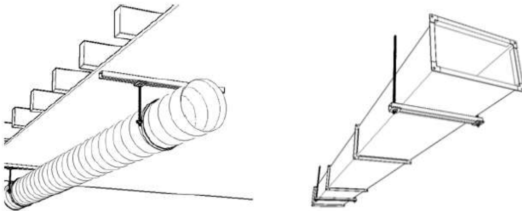
Duct Hanger
